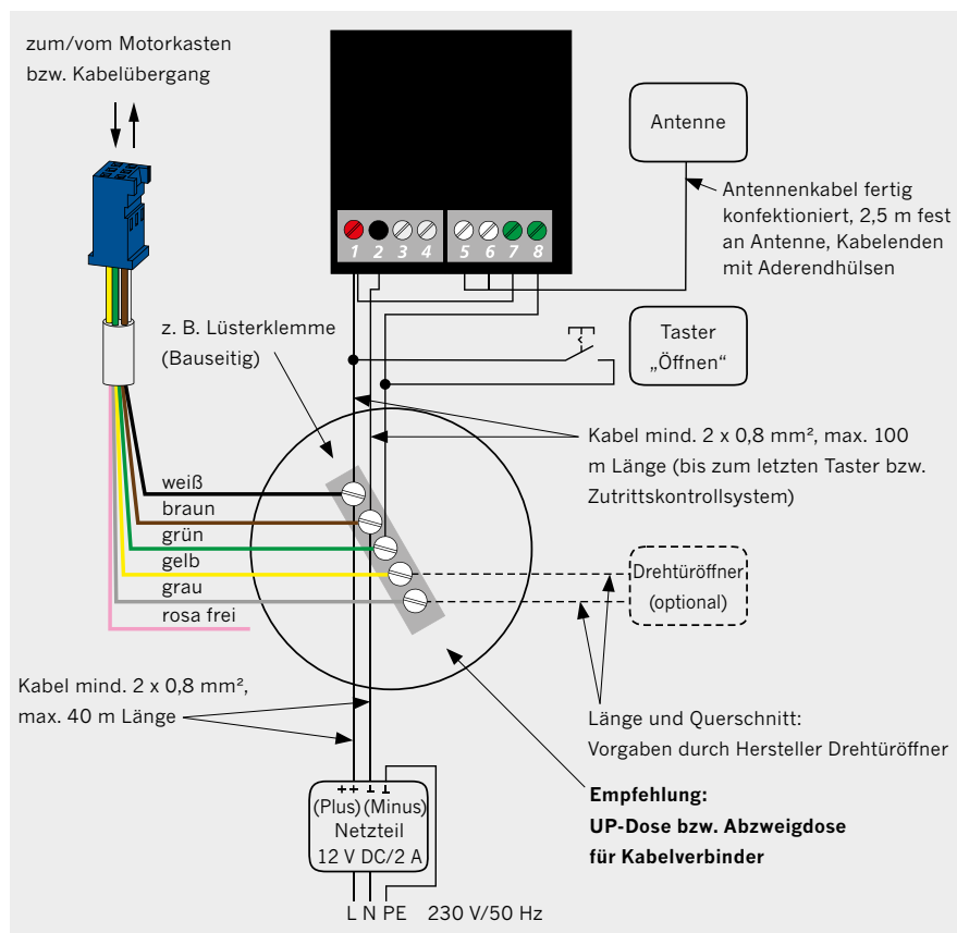
Abbildung 3.4-2: Installation Transponder-Leser
